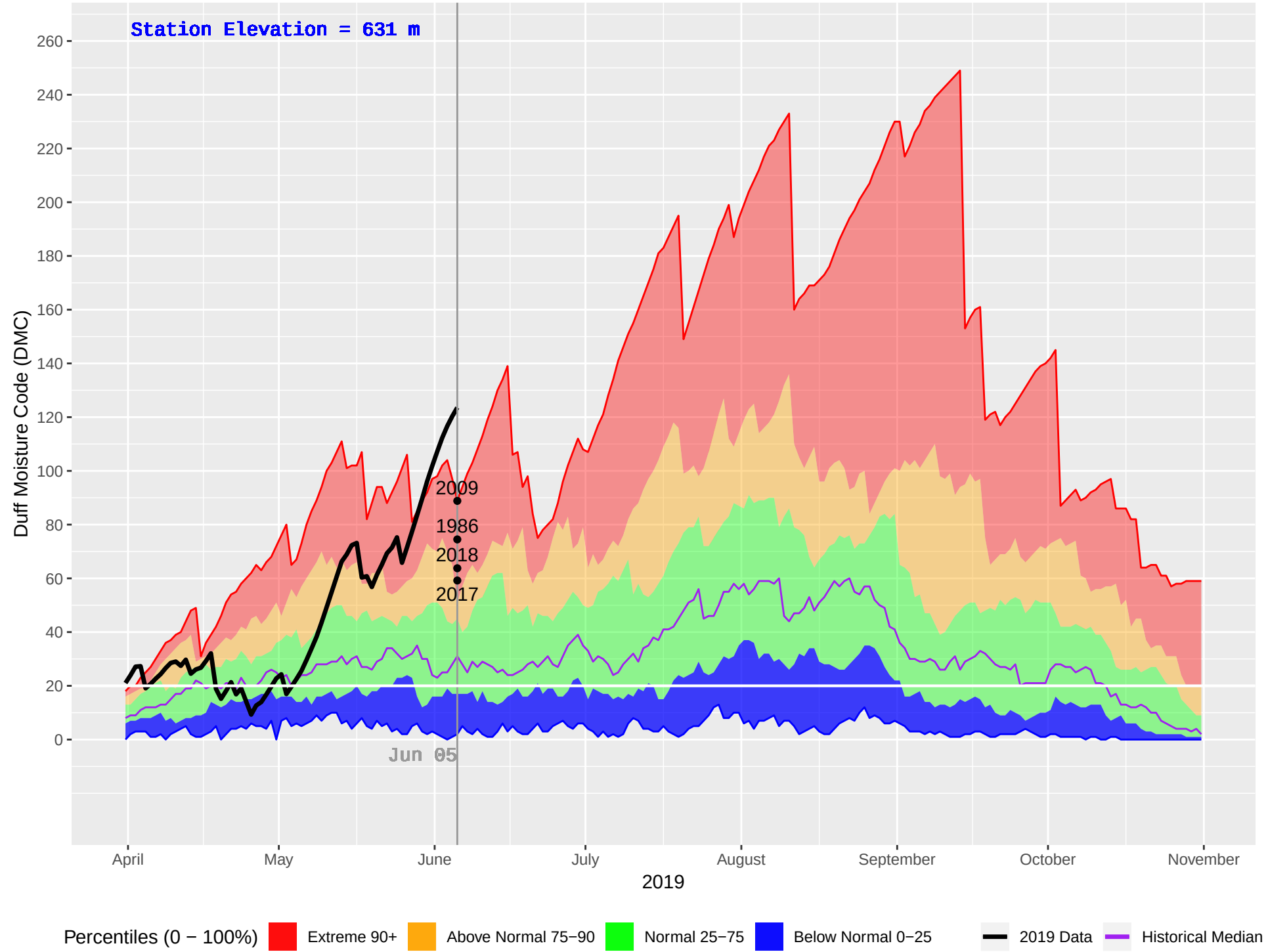
EAST BARRIERE (243) : Historical (1978–2018), Current (2019) Daily Duff Moisture Code (DMC)
