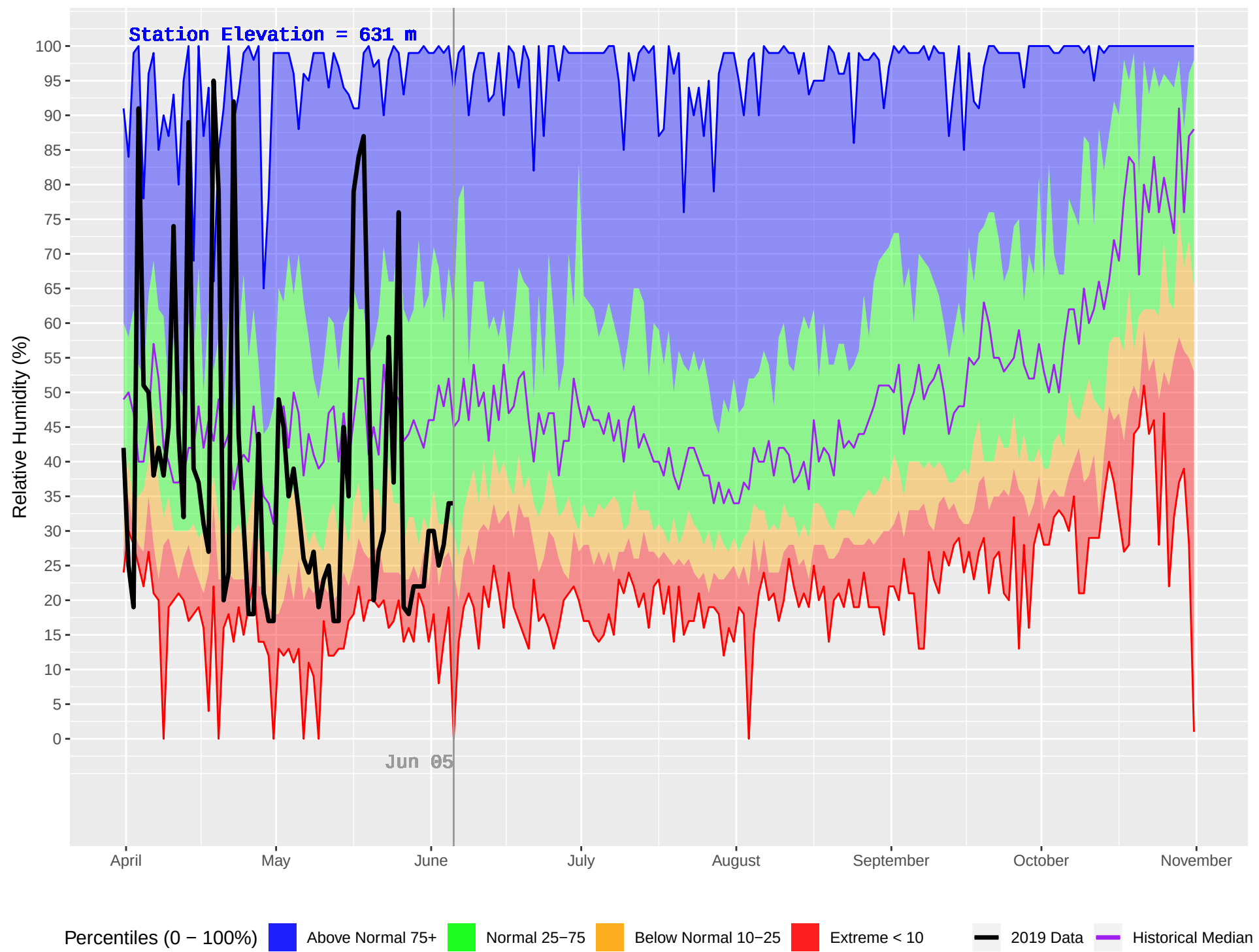
EAST BARRIERE (243) : Historical (1978–2018) and Current (2019) Daily Relative Humidity
