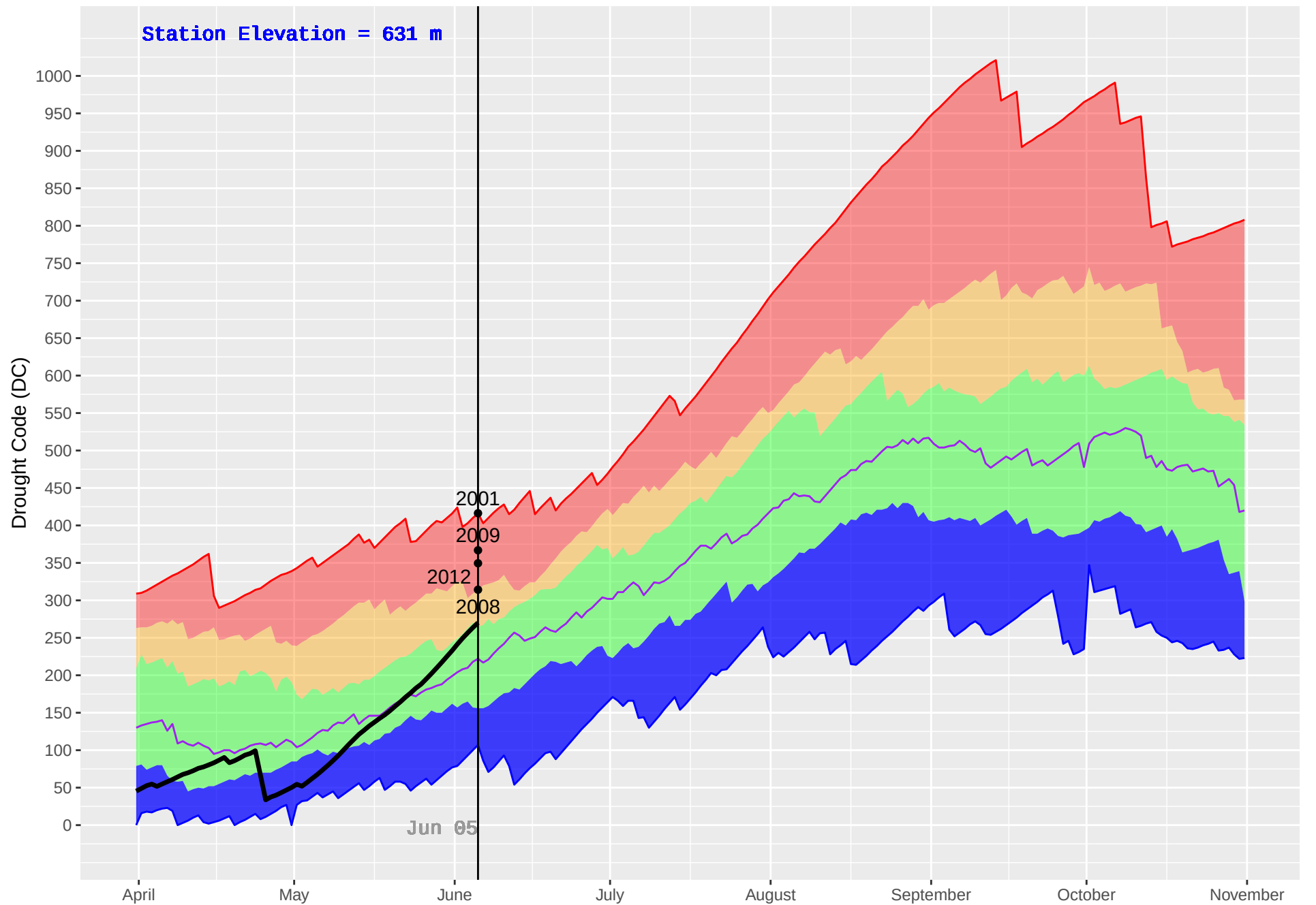
EAST BARRIERE (243) : Historical (1978–2018) and Current (2019) Daily Drought Code (DC)
