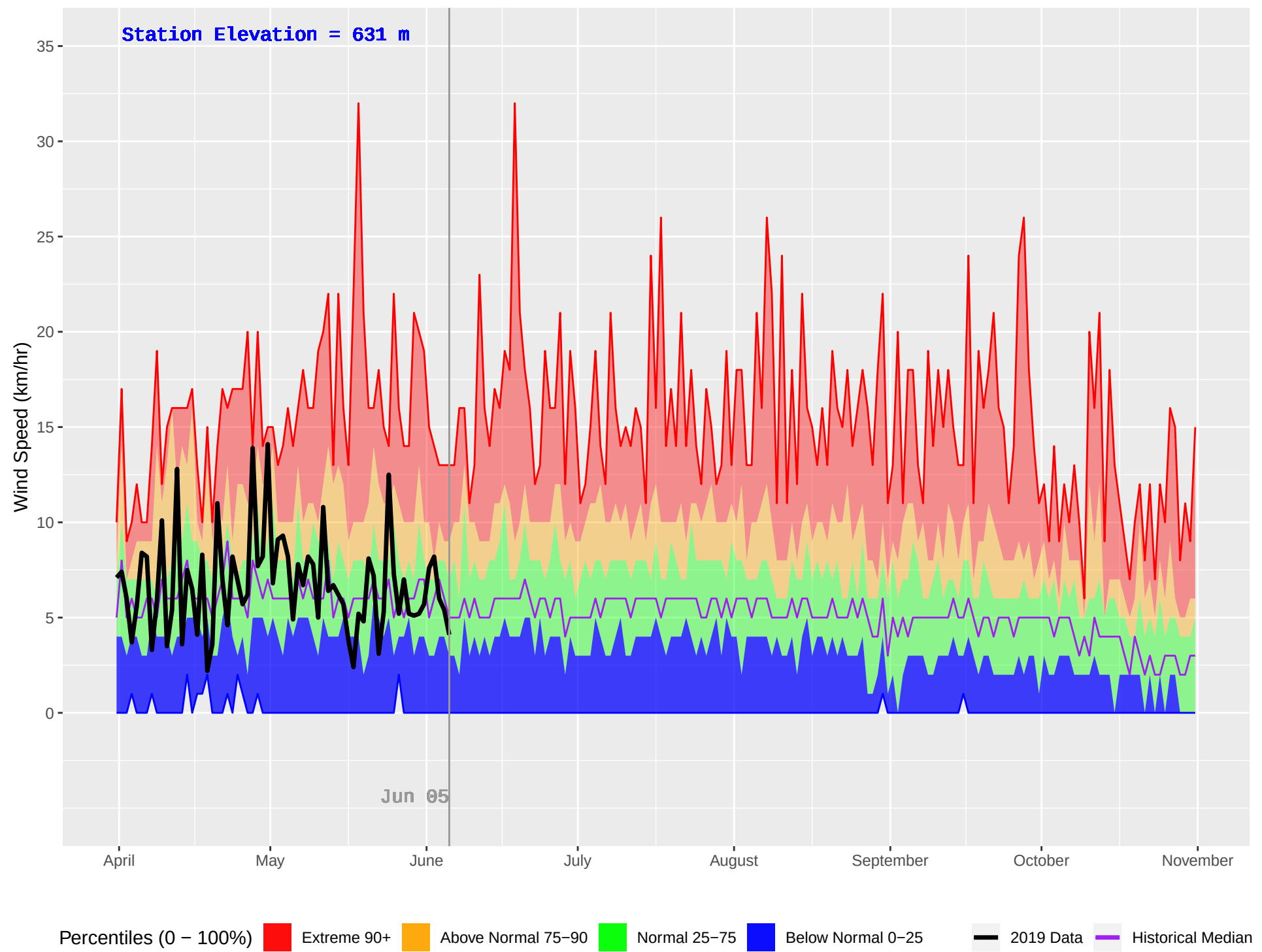
EAST BARRIERE (243) : Historical (1978–2018) and Current (2019) Daily Wind Speed
