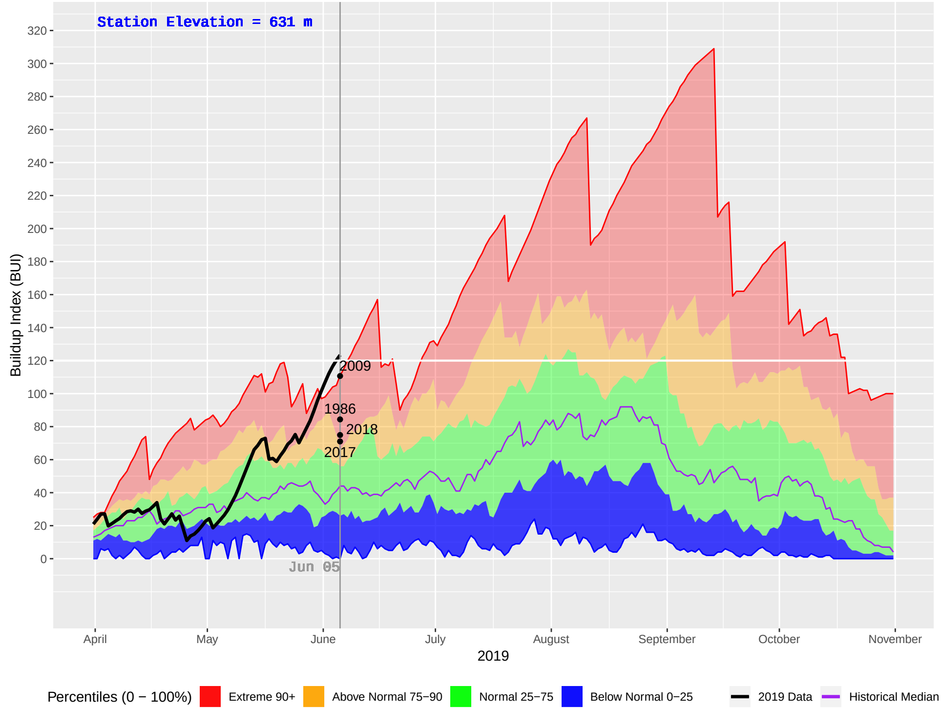
EAST BARRIERE (243) : Historical (1978–2018), Current (2019) Daily Buildup Index (BUI)
