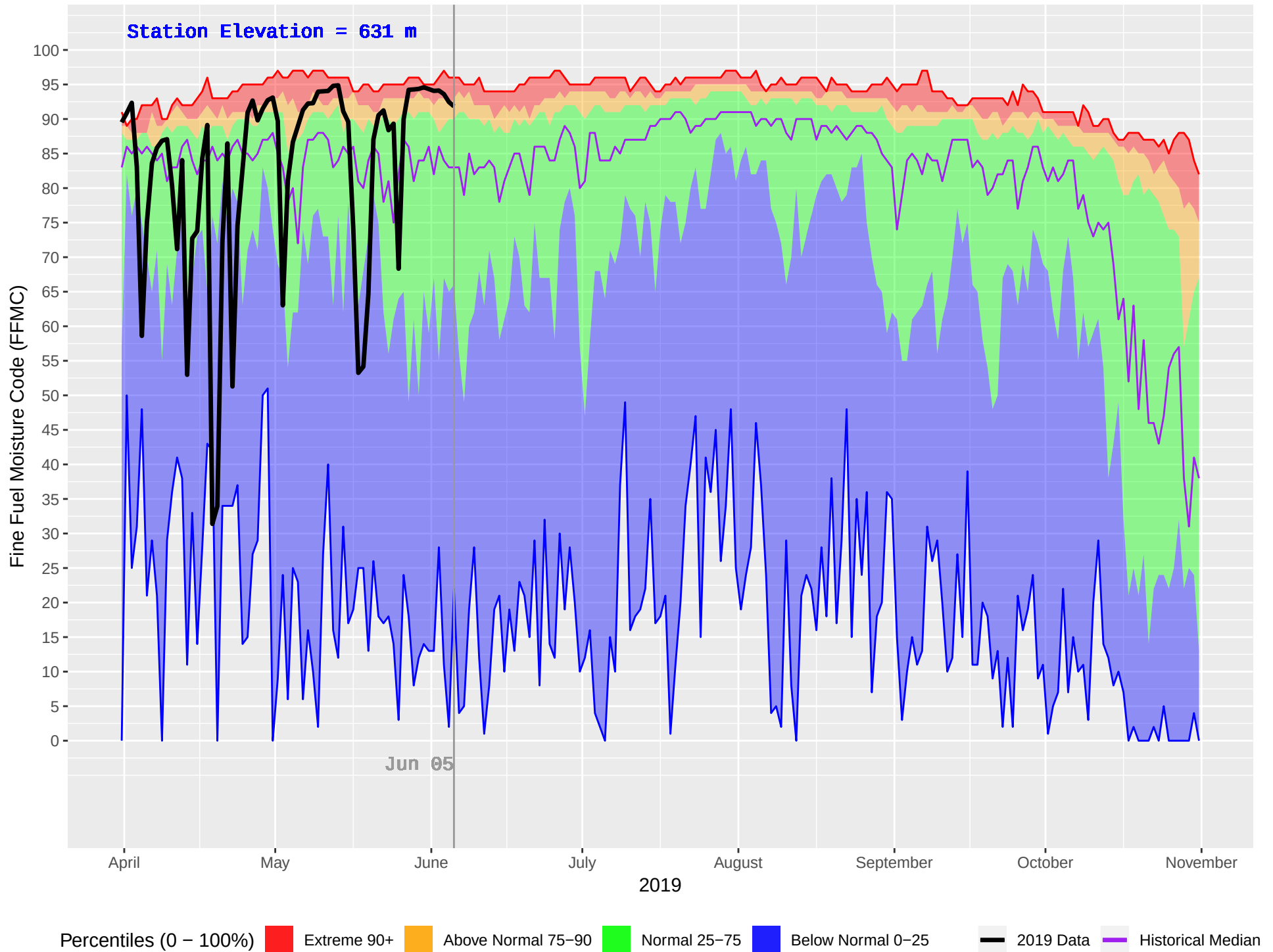
EAST BARRIERE (243) : Historical (1978–2018) and Current (2019) Daily Fine Fuel Moisture Code (FFMC)
