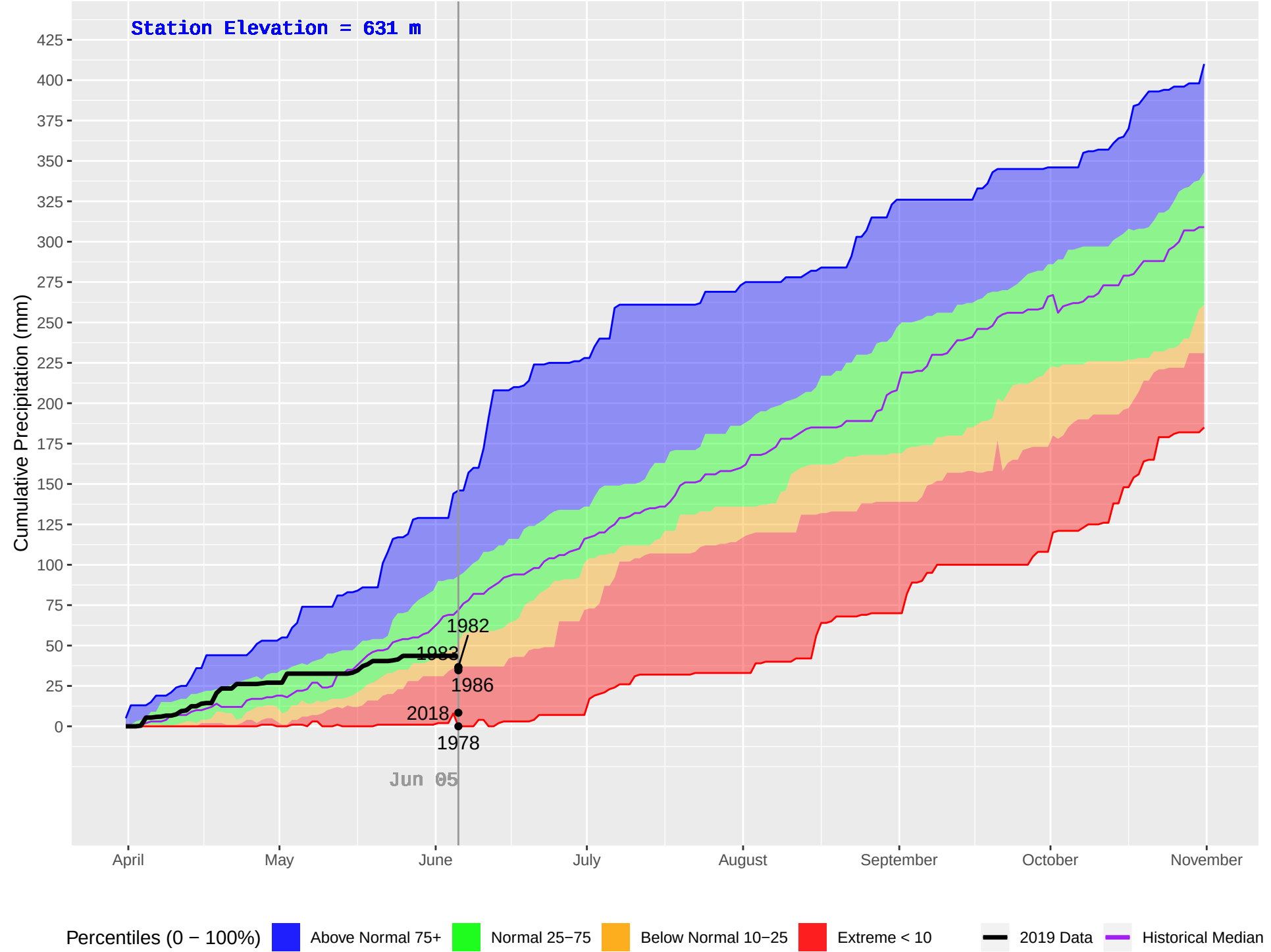
EAST BARRIERE (243) : Historical (1978–2018), Current (2019) Daily Cumulative Precipitation
